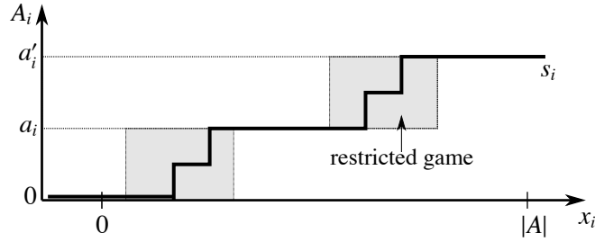
FIGURE 2. Exploiting the GGS of restricted games
