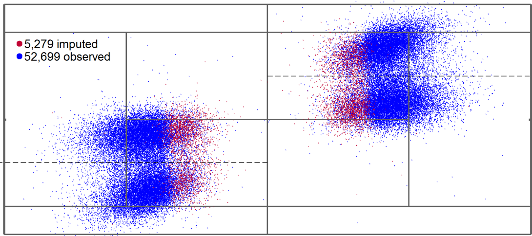
Figure C5: Ball Bounces for Deuce Court First Serves by Women
