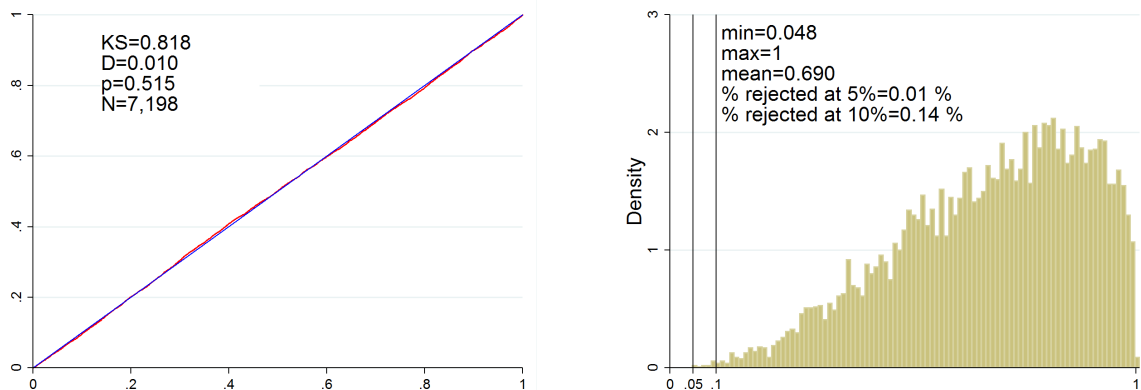
(a) An empirical c.d.f. of t -values (b) Density of KS test p -values (10,000 trials)
