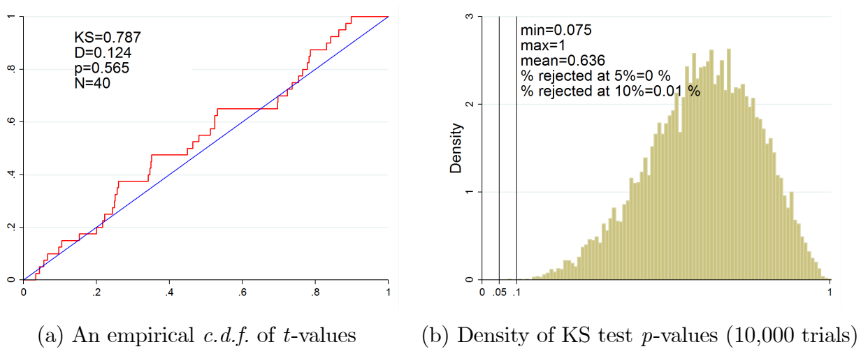
Figure 15: KS test of H_0 : p_L^i = p_R^i \forall i (WW data)
