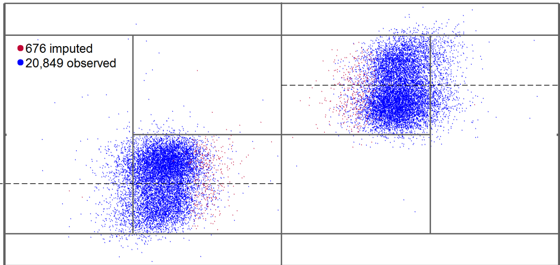
Figure C6: Ball Bounces for Deuce Court Second Serves by Women
