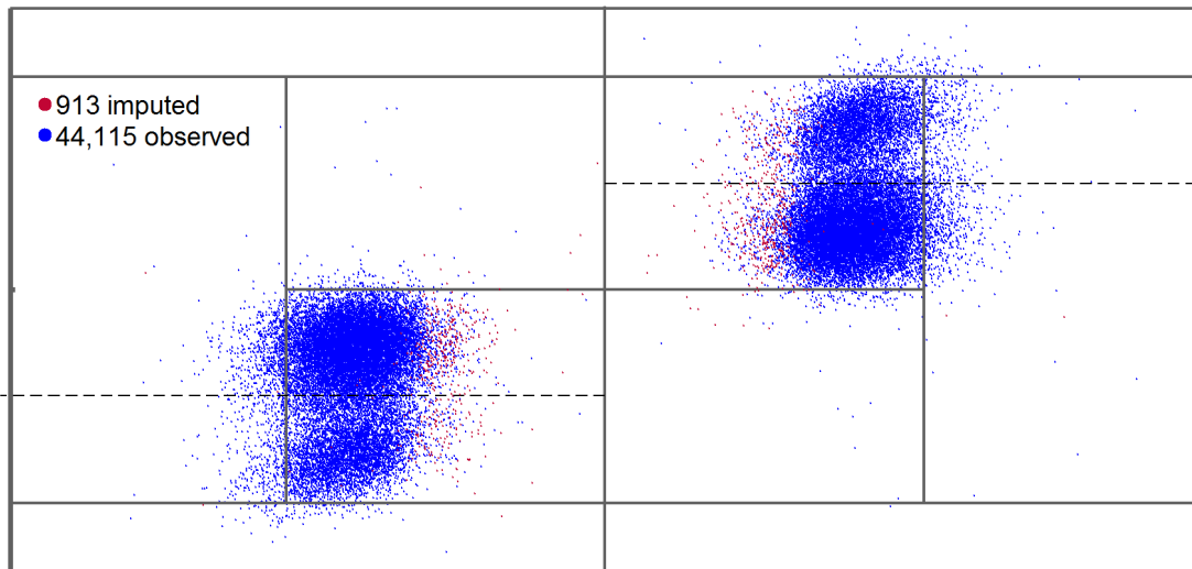
Figure C2: Ball Bounces for Deuce Court Second Serves by Men
