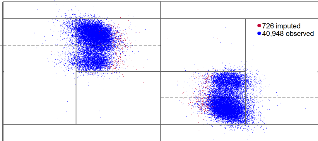
Figure C4: Ball Bounces for Ad Court Second Serves by Men
