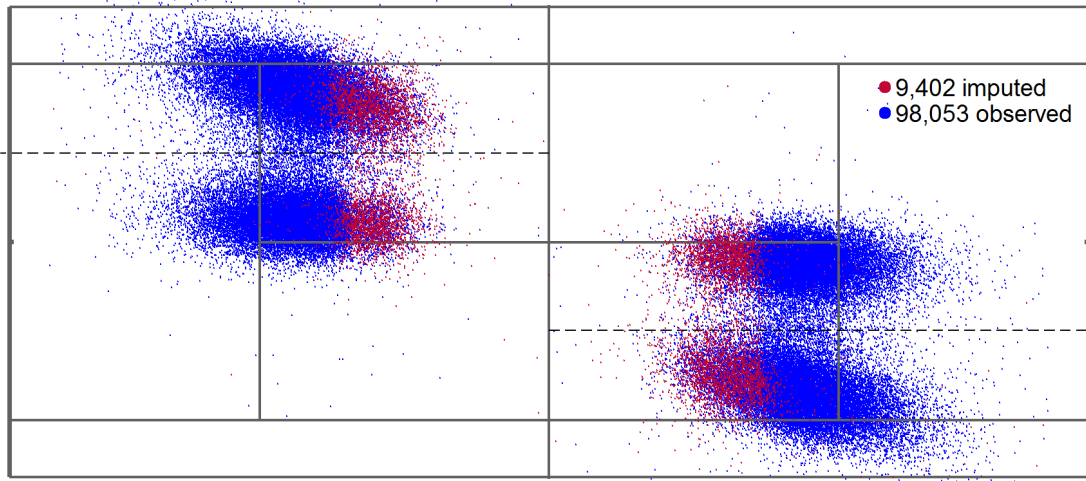
Figure C3: Ball Bounces for Ad Court First Serves by Men
