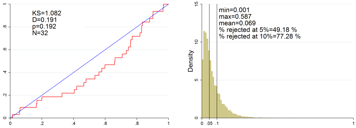
Figure 16(c): KS test for Juniors of H_0 : p_L^i = p_R^i \forall i (HHT data)
