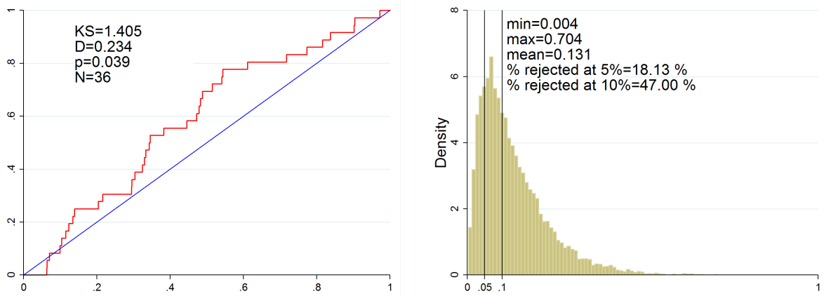
Figure 16(b): KS test for Women of H_0 : p_L^i = p_R^i \forall i (HHT data)
