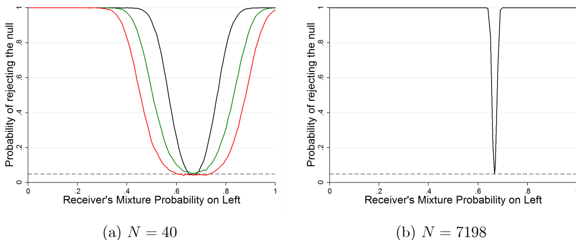
Figure C1: Power Functions for KS test based on t -values (black), p -values (red), and Pearson joint (green)
