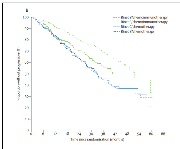
Figure 1: Progression-free survival in the CLL-8 trial by treatment and Binet stage
