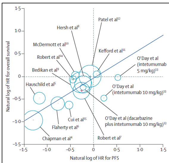
Figure 3: Correlation between treatment effects on overall survival and PFS
