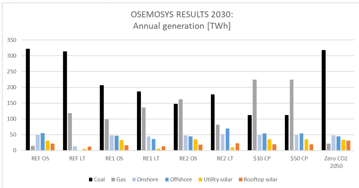
Figure 41: Viet Nam: Annual generation under various scenarios (2030)
