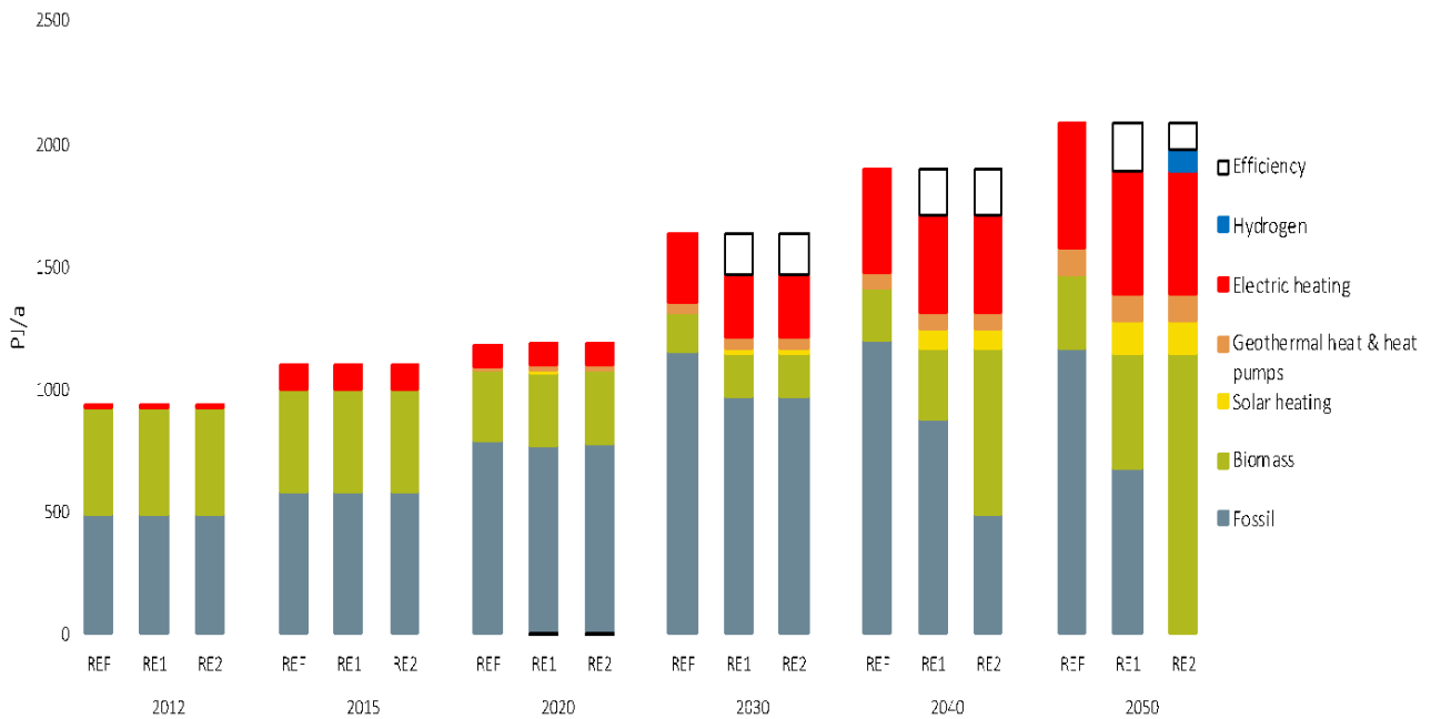
Figure 20: Projection of heat supply by energy carrier (REF, RE1, and RE2)
