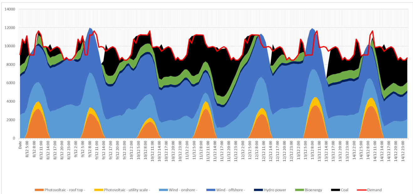
Figure 37: Red River Delta—example of very high renewable electricity production (16 th to 23 th May 2030)
