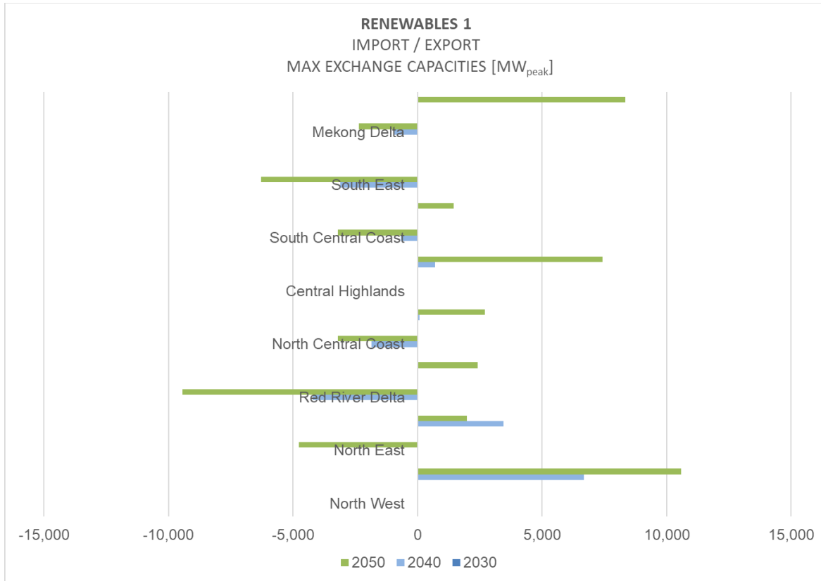
Figure 32: Viet Nam: Maximum interregional exchange capacities—additional to the required grid capacity expansion in response to load increase—under the RENEWABLES 1 scenario
