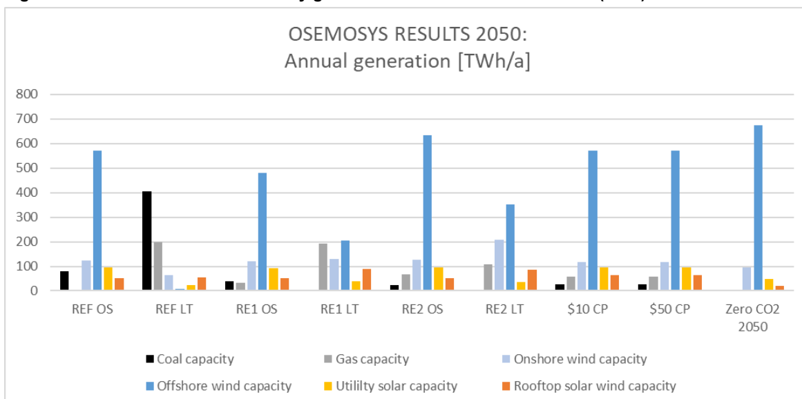
Figure 43: Viet Nam: Annual electricity generation under various scenarios (2050)
