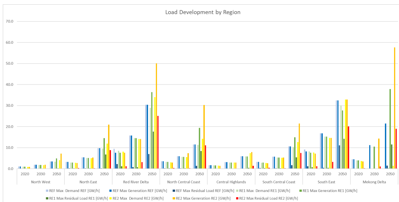
Figure 34: Peak load and maximum generation development by region, in GW
