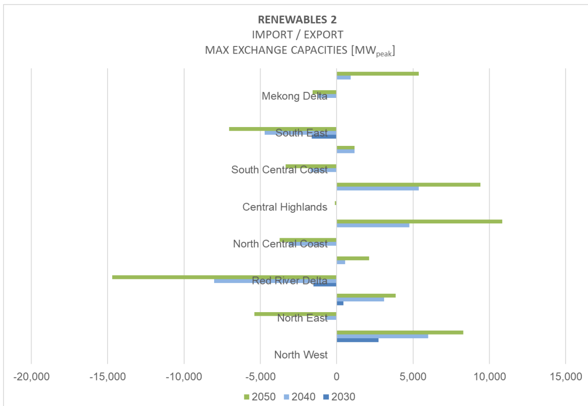
Figure 33: Viet Nam: Maximum interregional exchange capacities—additional to the required grid capacity expansion in response to load increase—under the RENEWABLES 2 scenario
