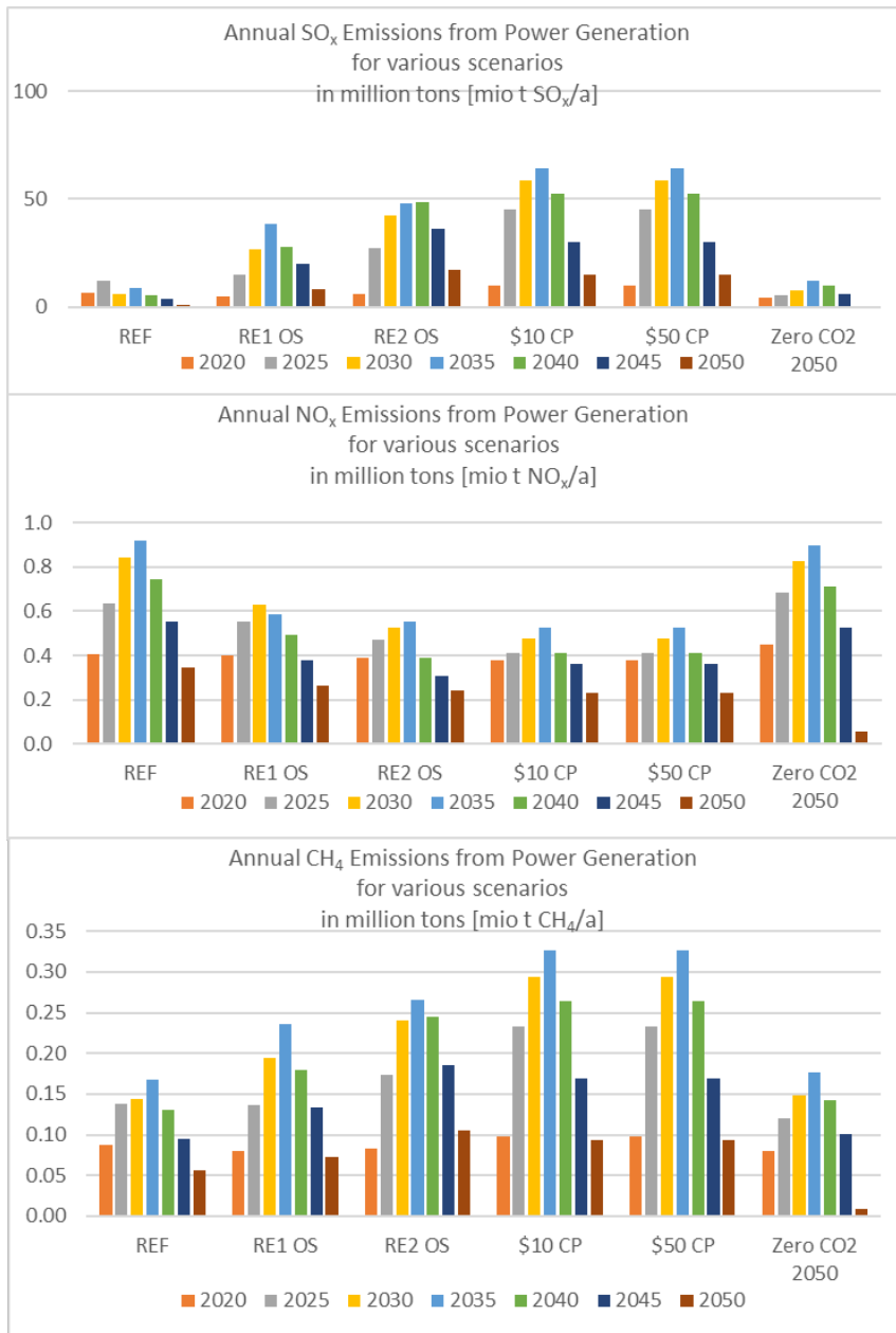
Figure 46: Viet Nam: Comparison of annual SO x , NO x , and CH 4 emissions from power generation under various scenarios
