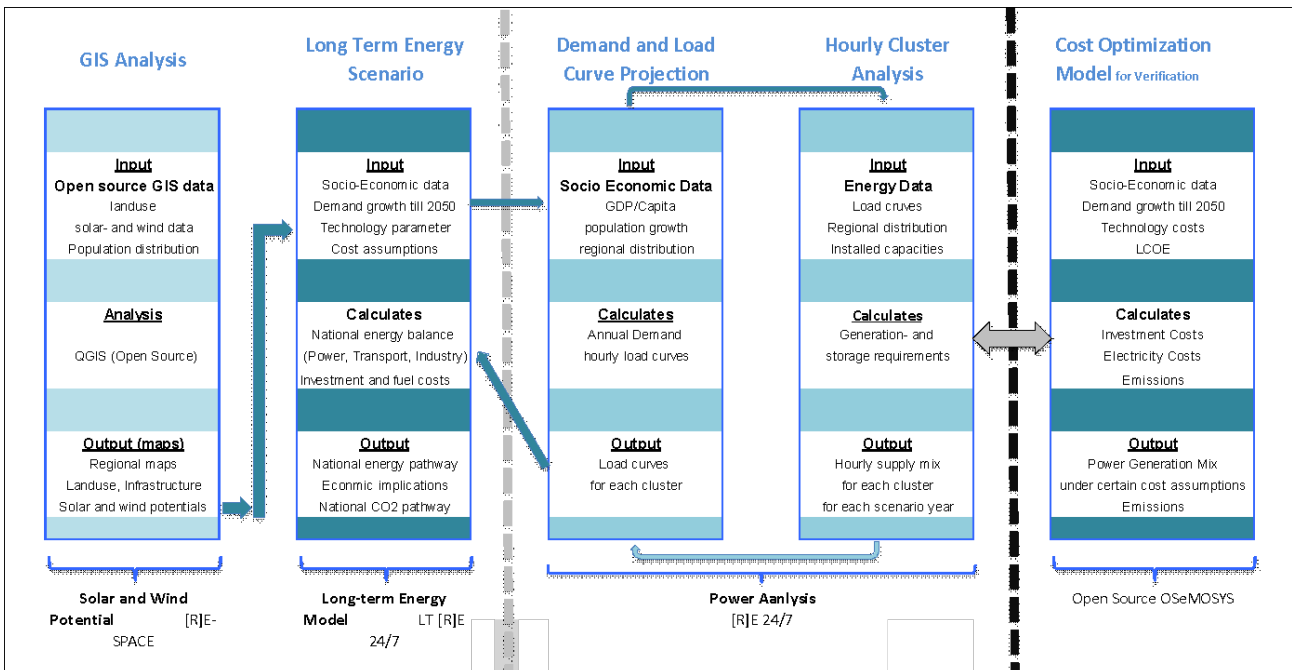
Figure 3: Overview—Modelling concept
