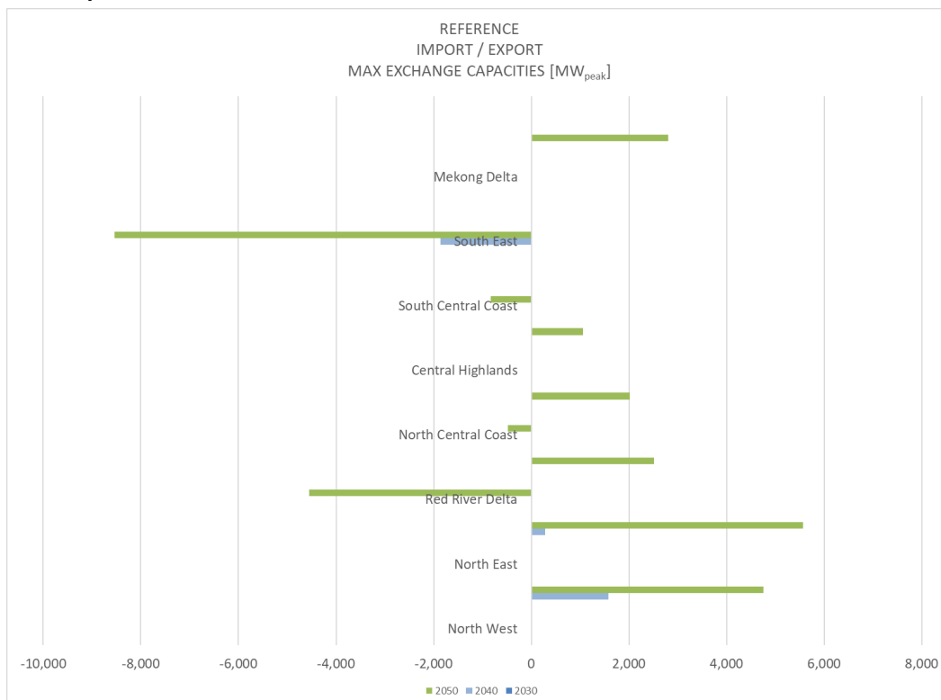
Figure 31: Viet Nam: Maximum interregional exchange capacities—additional to the required grid capacity expansion in response to load increase—under the REFERENCE scenario
