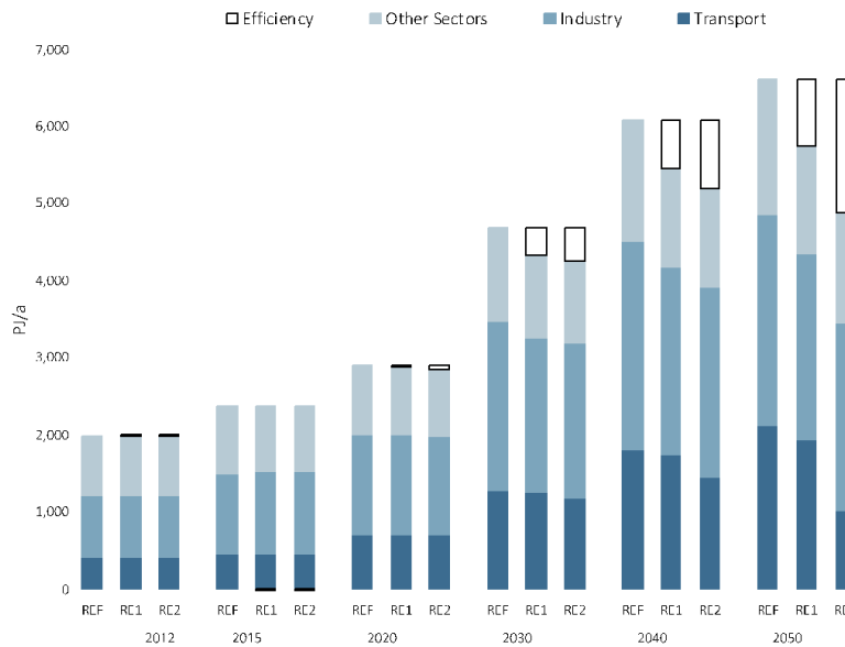
Figure 16: Projection of total final energy demand by sector (excluding non-energy use and heat from CHP auto-producers)
