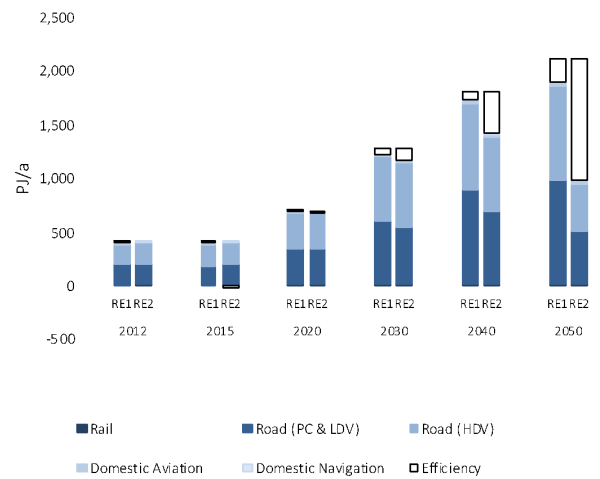
Figure 18: Development of the final energy demand for transport by sector in the RENEWABLES scenarios
