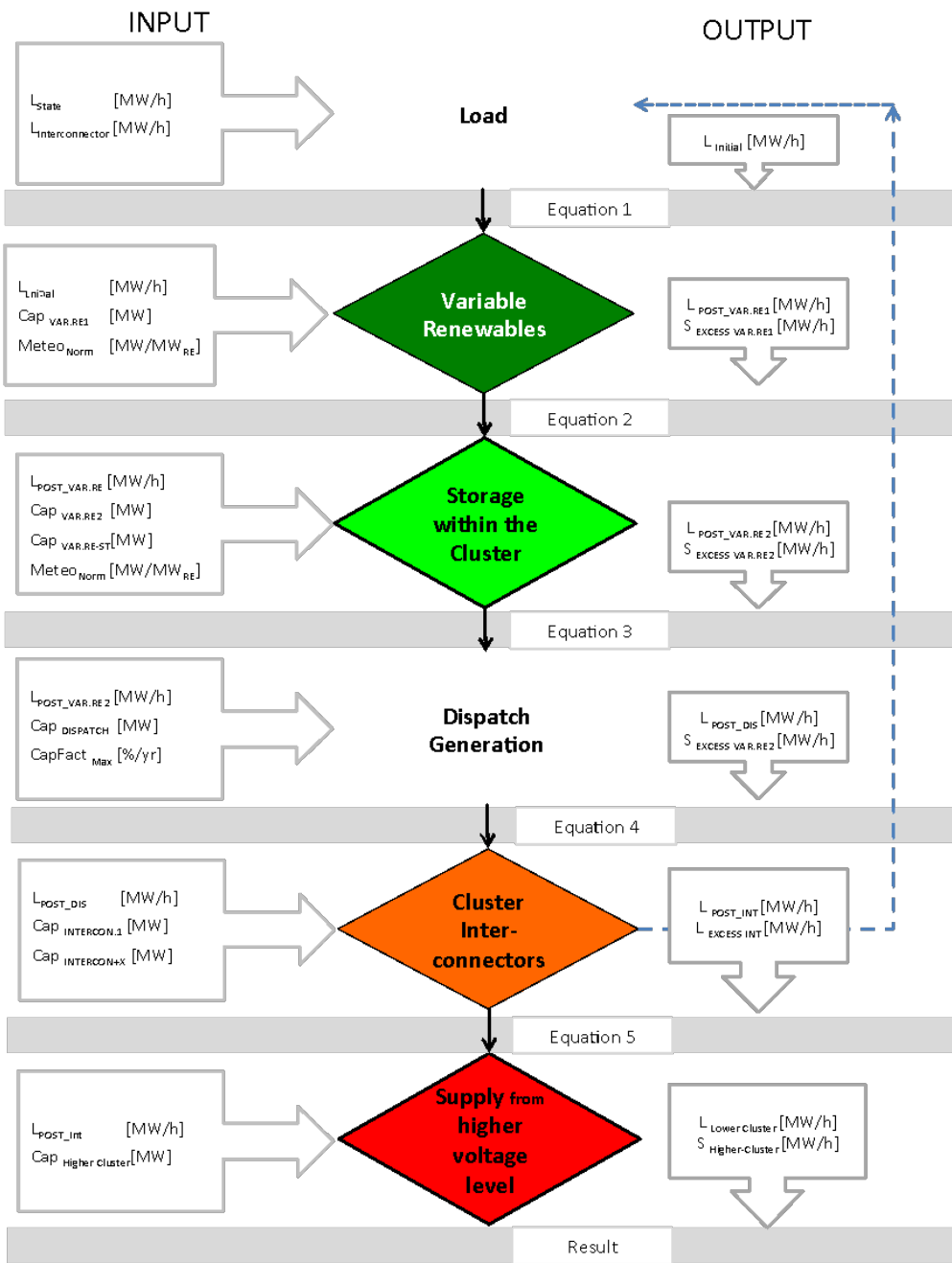
Figure 6: Overview—input, output, and dispatch order
