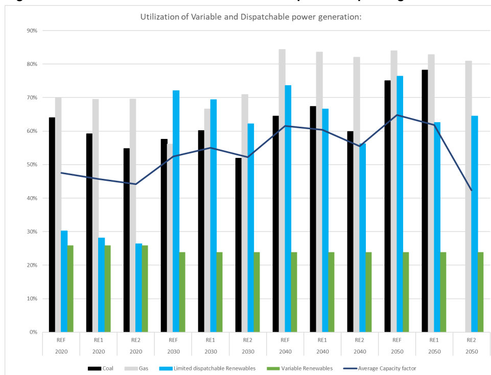
Figure 30: Viet Nam: Utilization of variable and dispatchable power generation
