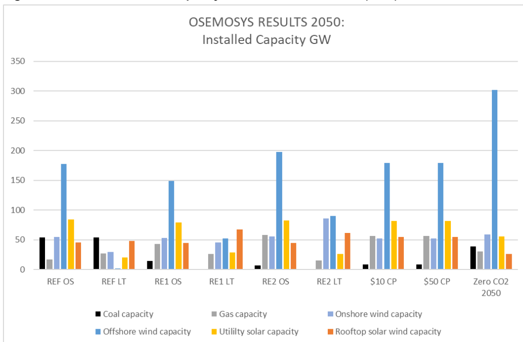
Figure 42: Viet Nam: Installed capacity under various scenarios (2050)
