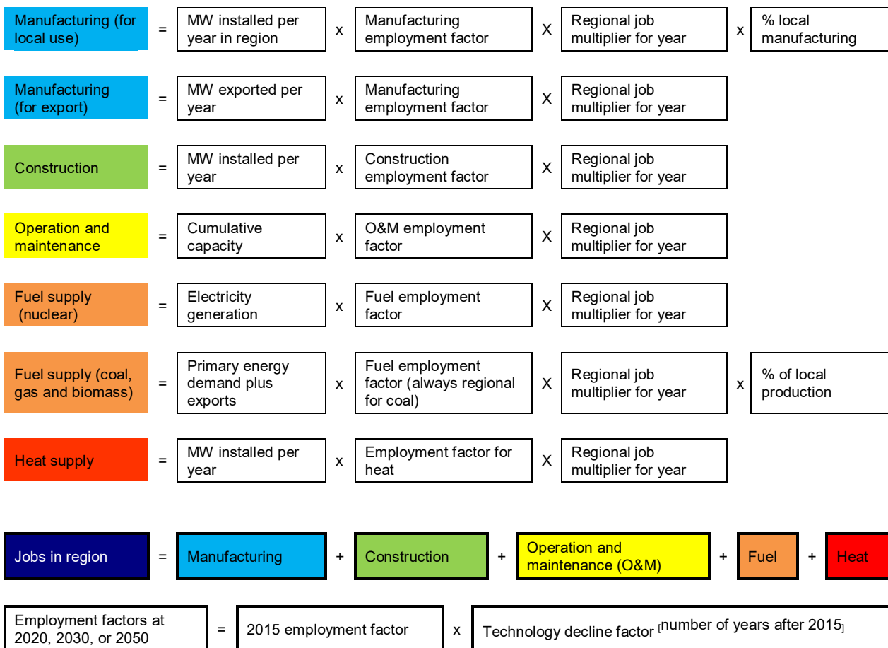
Figure 48: Total employment calculation: methodological overview
