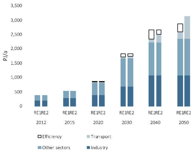
Figure 17: Development of the electricity demand by sector in both RENEWABLES scenarios
