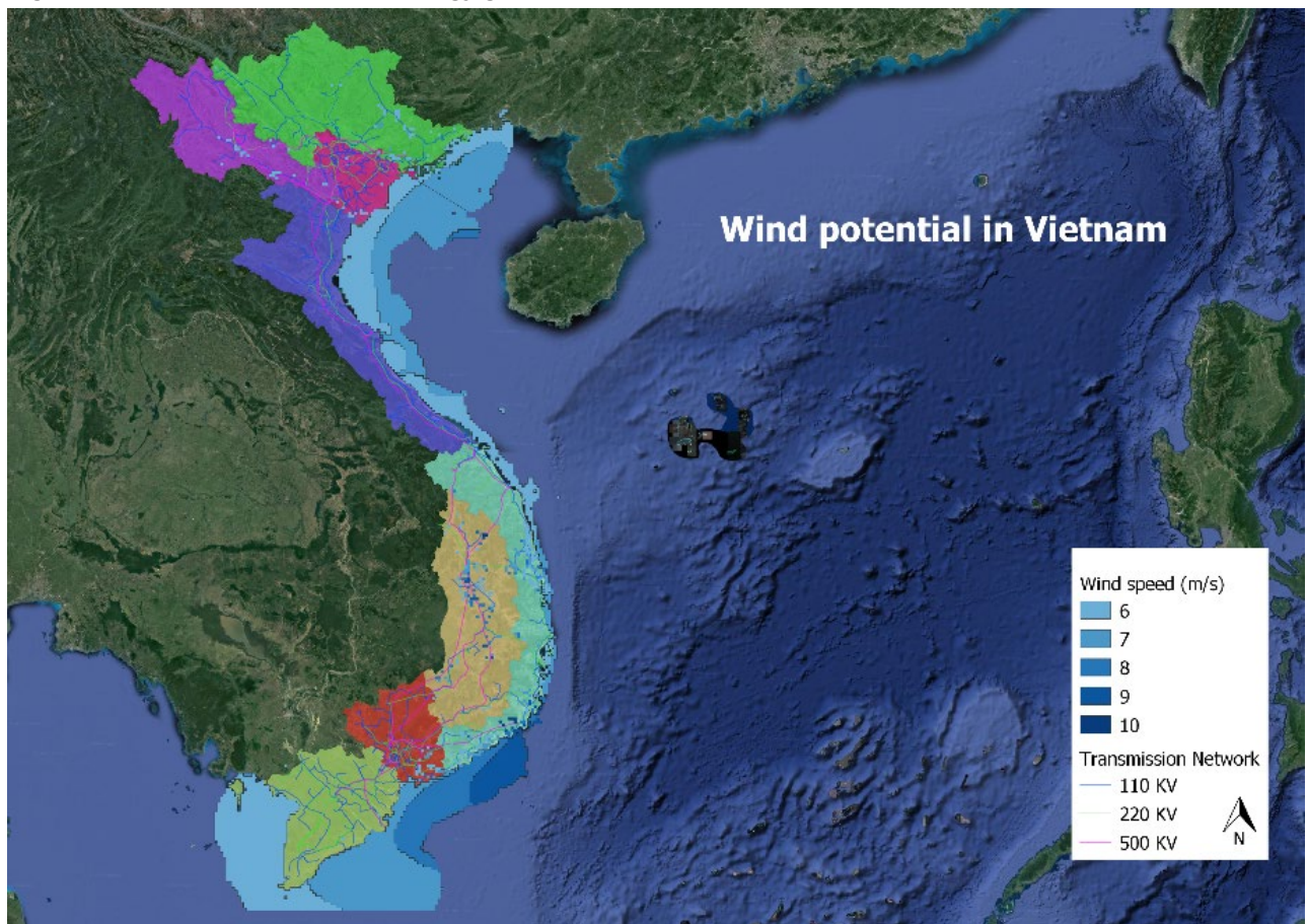
Figure 14: On- and offshore wind energy generation potential in Viet Nam
