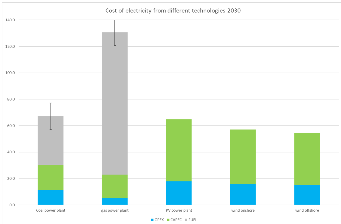
Figure 27: Costs of electricity generation with different technologies in 2030
