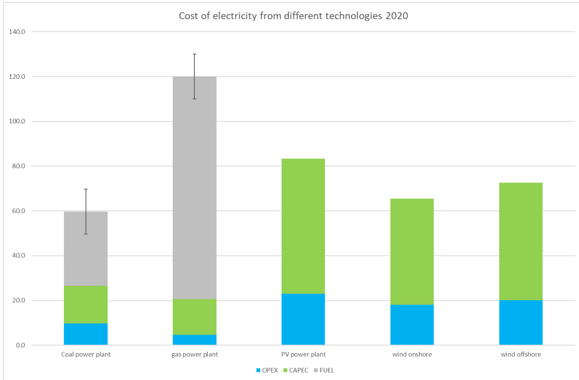
Figure 26: Costs of electricity generation with different technologies in 2020
