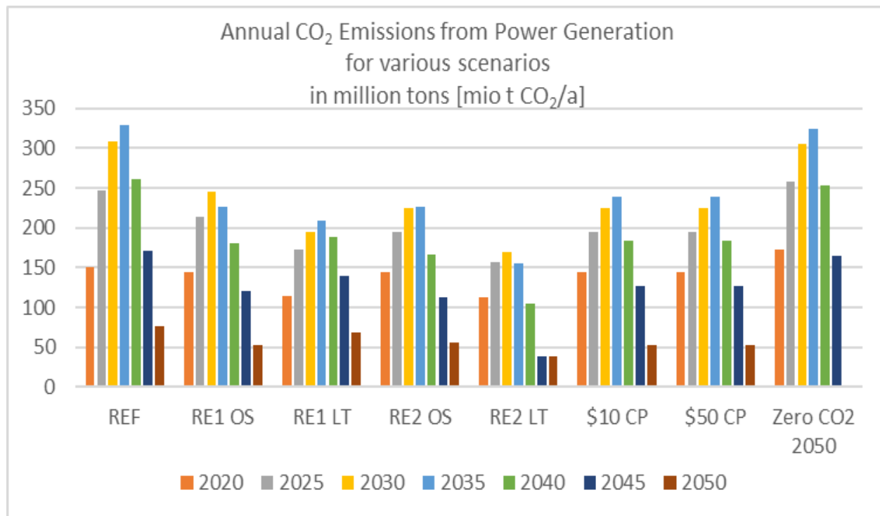
Figure 45: Viet Nam: Comparison of annual CO 2 emissions from power generation under various scenarios
