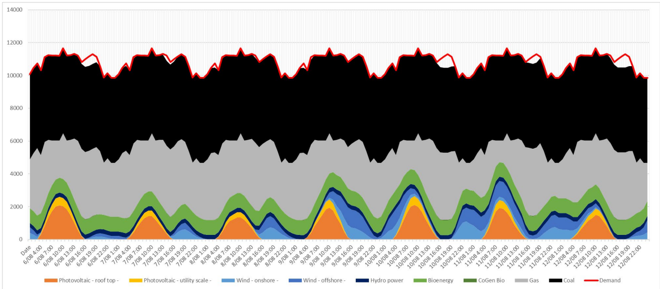
Figure 36: Red River Delta—example of very low renewable electricity production (6 th to 13 th August 2030)
