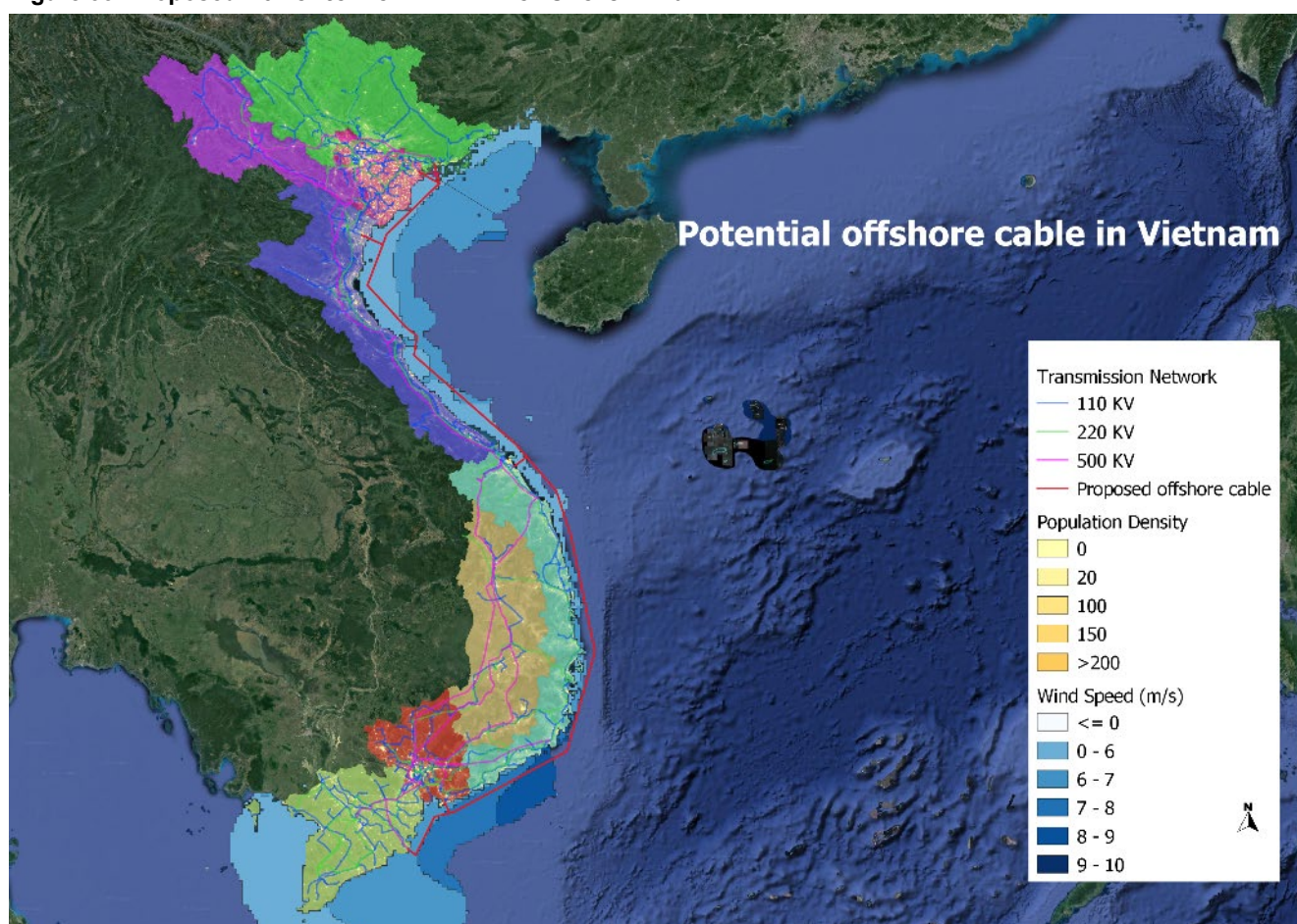
Figure 35: Proposed Hanoi to Ho Chi Minh offshore wind link
