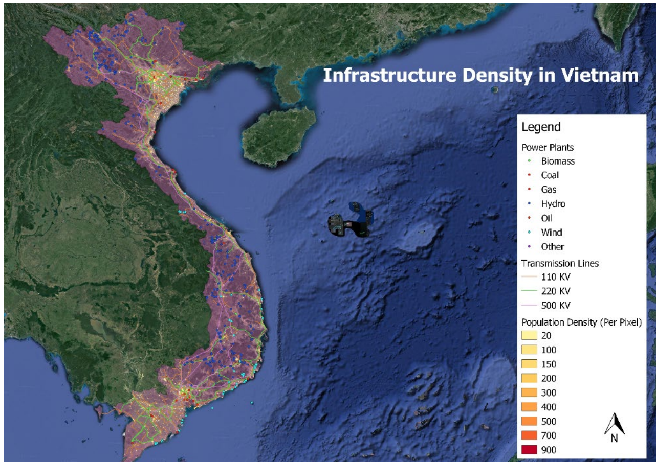
Figure 10: Existing electricity infrastructure by type
