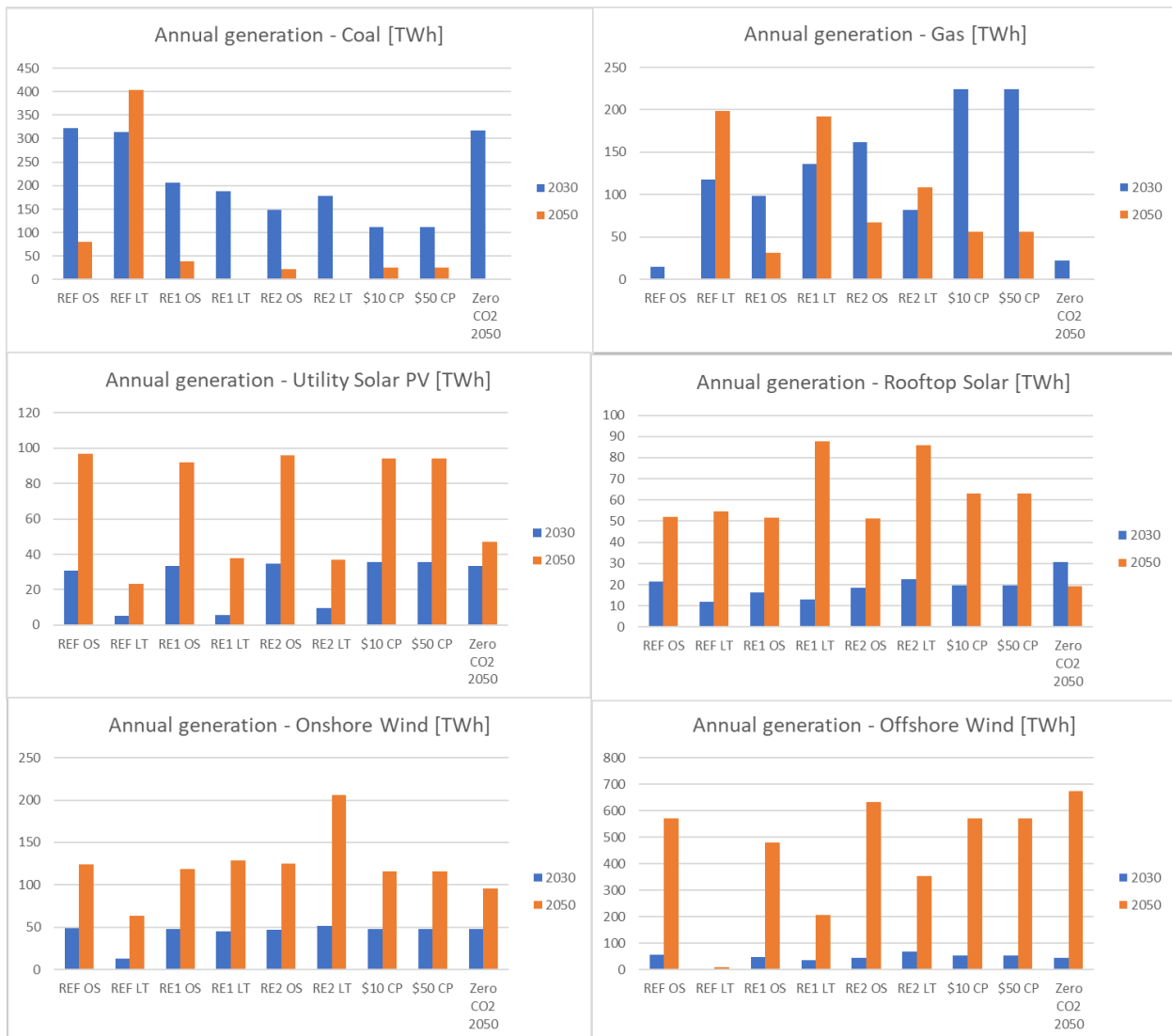
Figure 44: Viet Nam: Comparison of annual generation in 2030 versus 2050 under various scenarios
