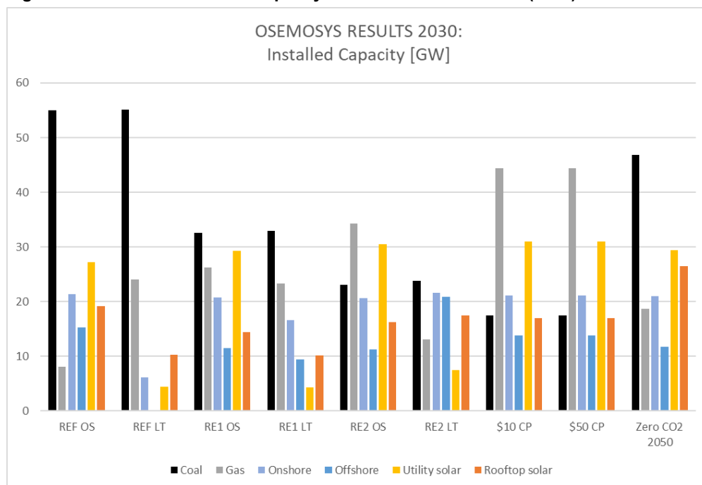
Figure 40: Viet Nam—Installed capacity under various scenarios (2030)
