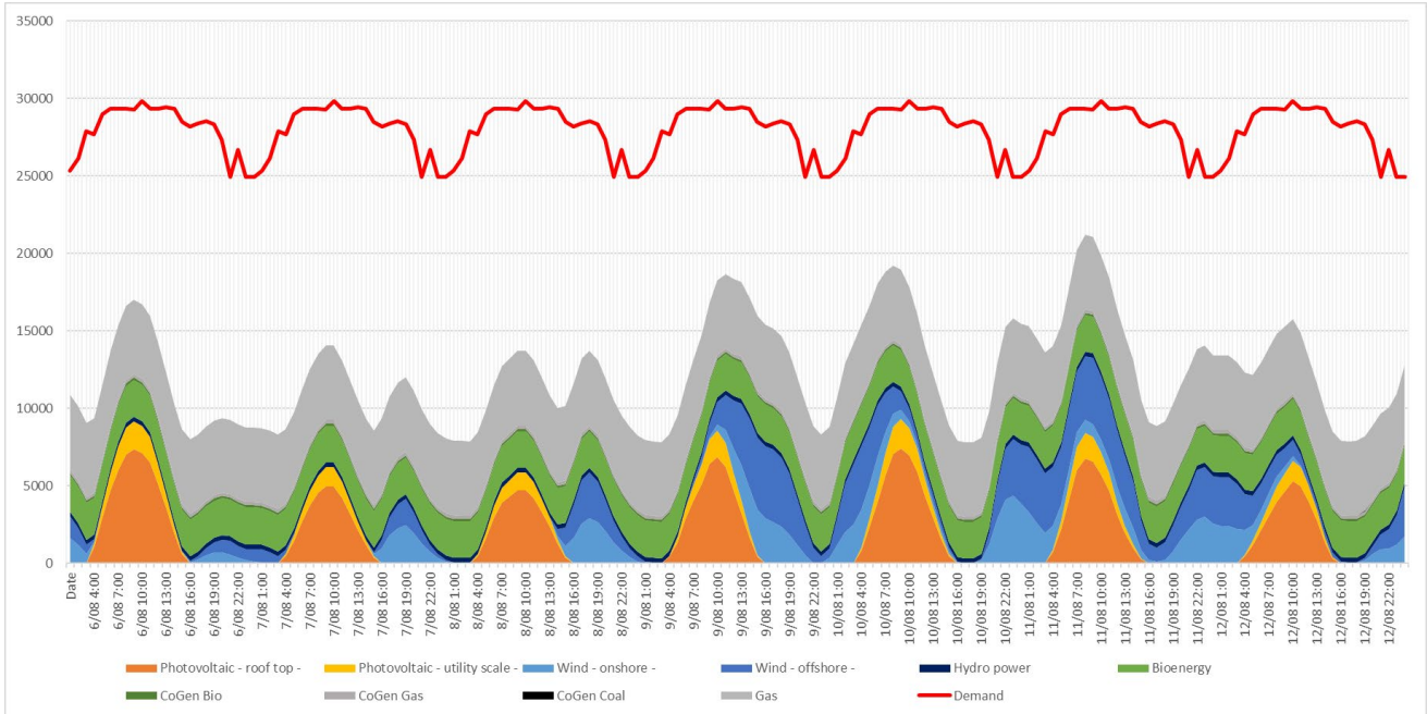
Figure 38: Red River Delta—example of very low renewable electricity production (6 th to 13 th August 2050)
